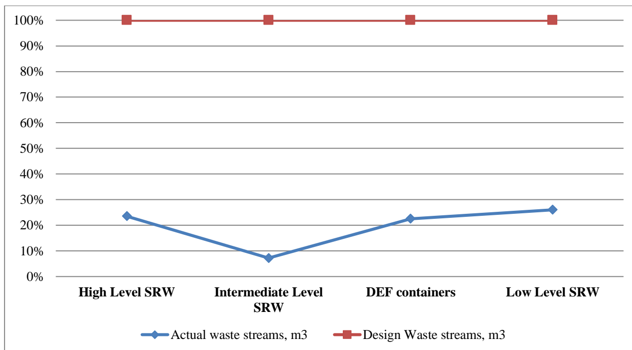
Figure 7. Design and annual SRW streams at the Armenian NPP
